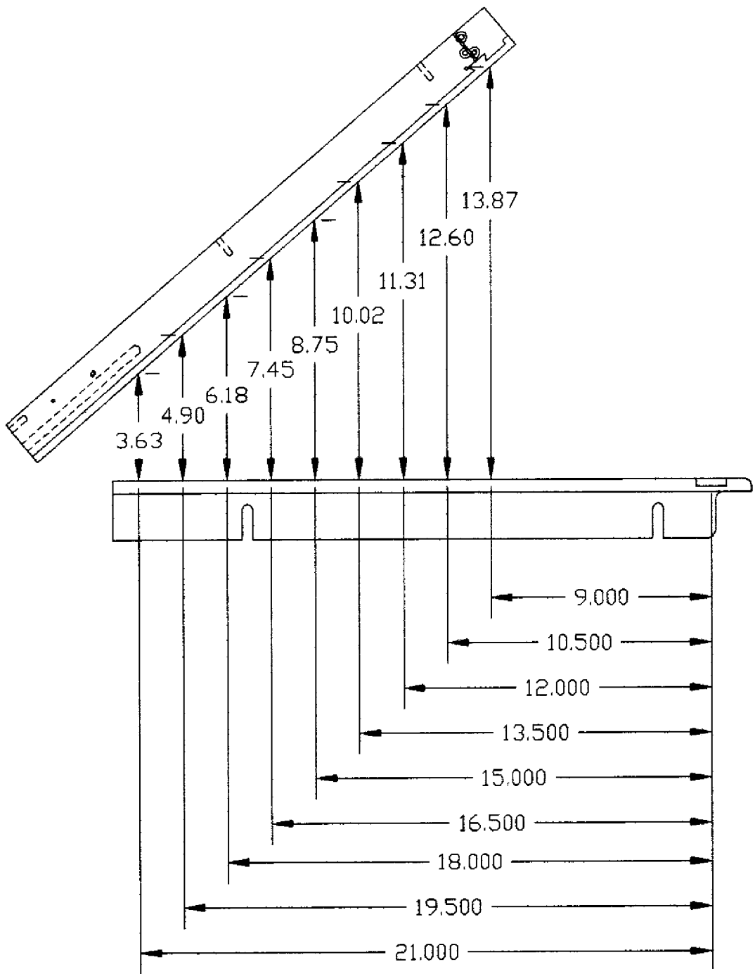
EP Hot Knife with a 20" side seal
