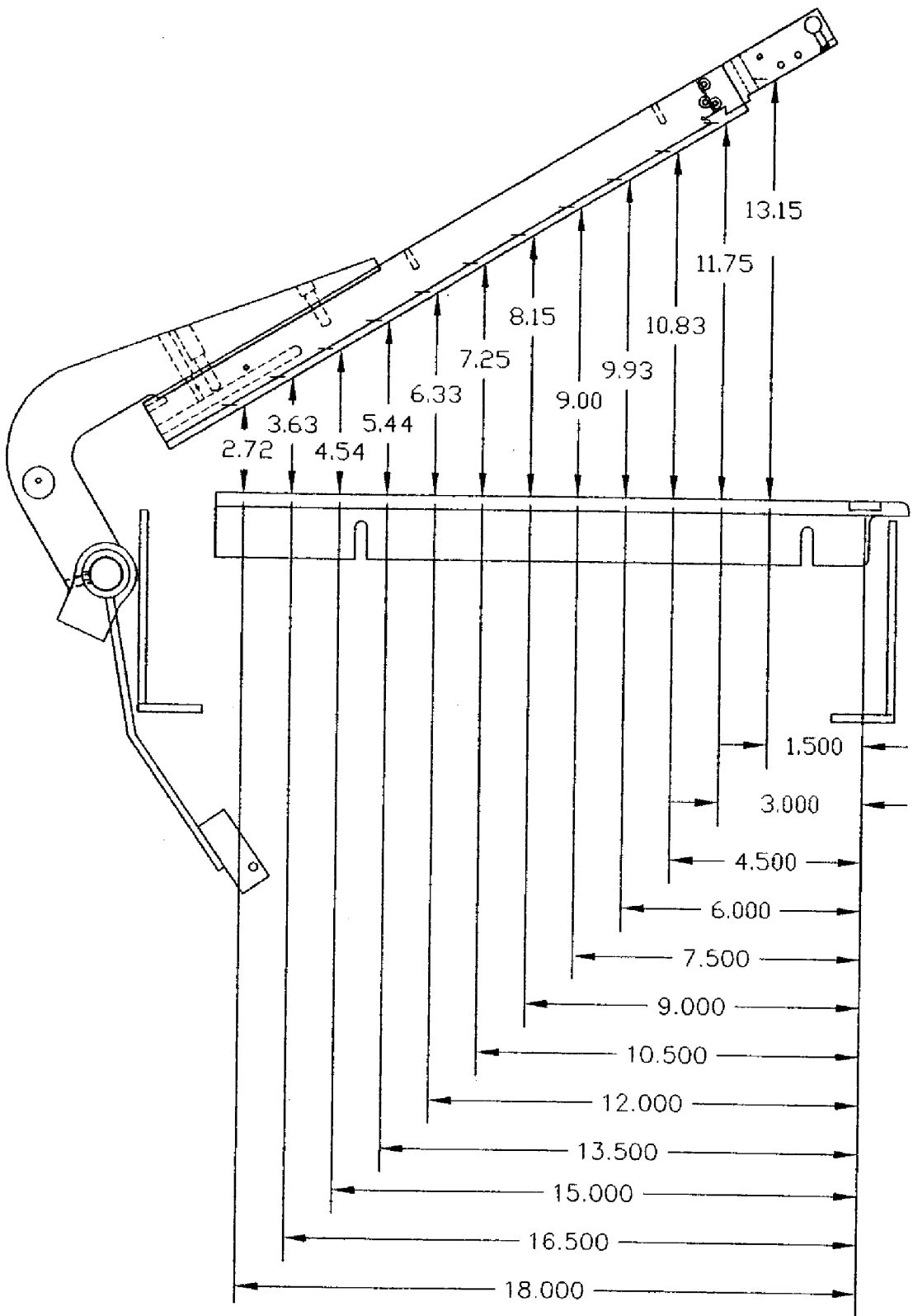
20" side seal Hot Knife
